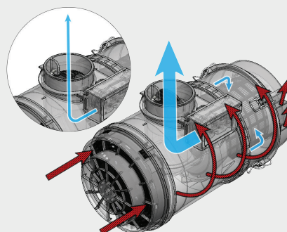
RESPA IQ Valve
